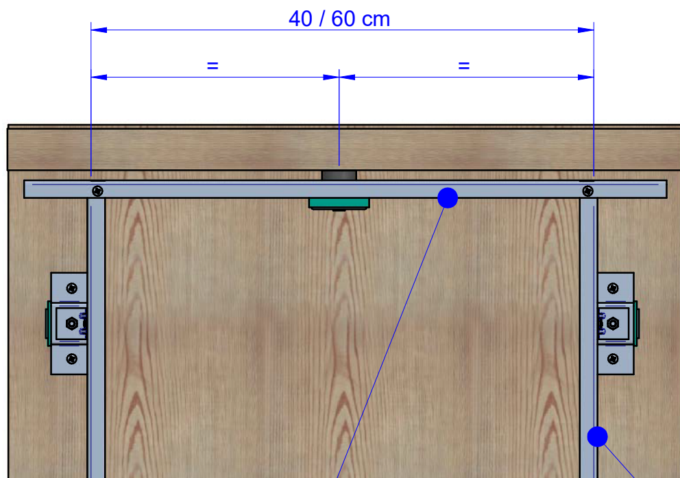
U-CHANNEL
