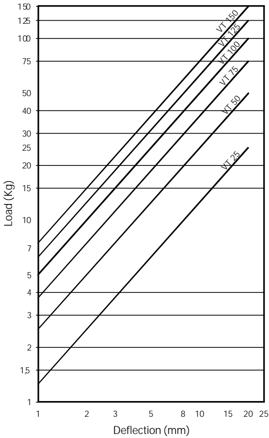
LOAD DEFLECTION CURVES VT TYPE 3 HANGERS
