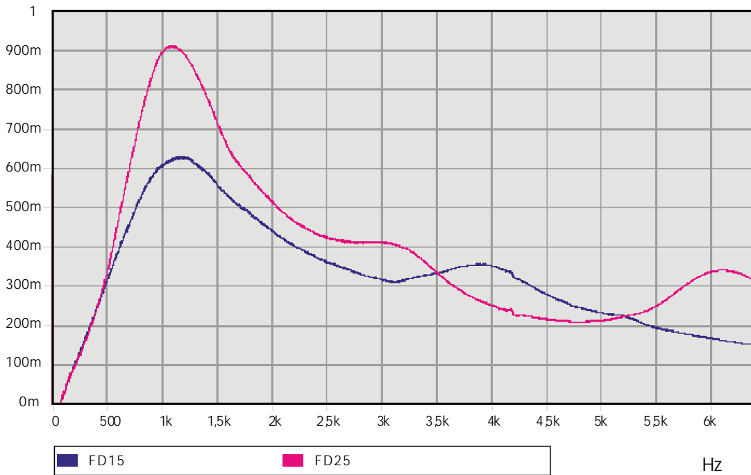
Absorption coefficient
