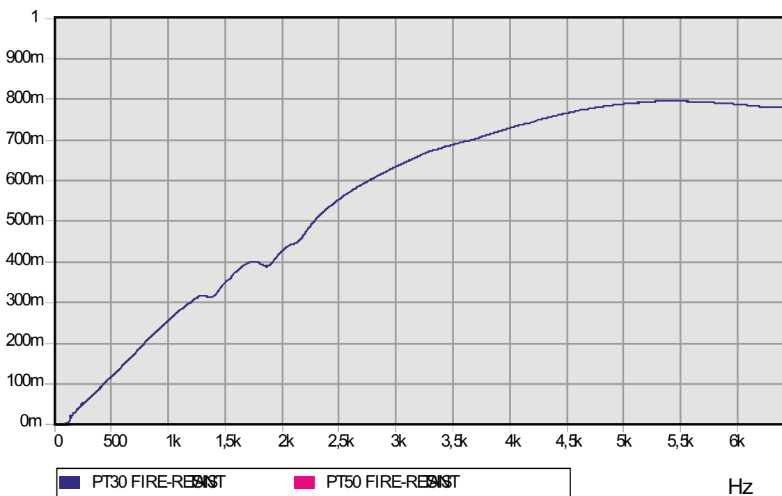
Absorption coefficient
