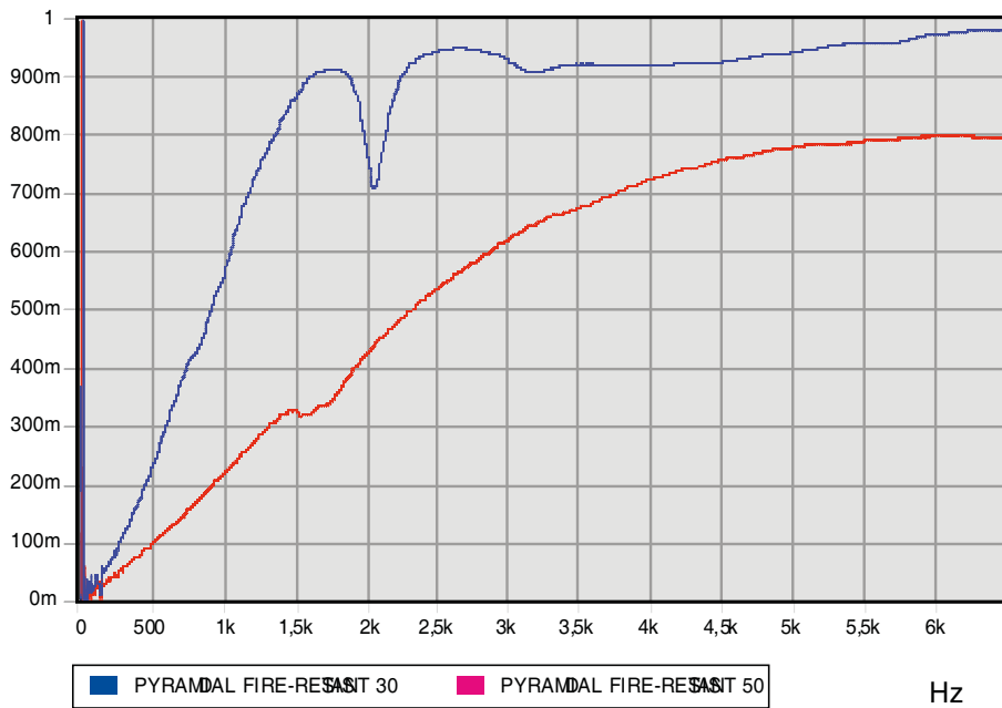
Absorption coefficient PYRAMDAL FIRE-RESIST 30
