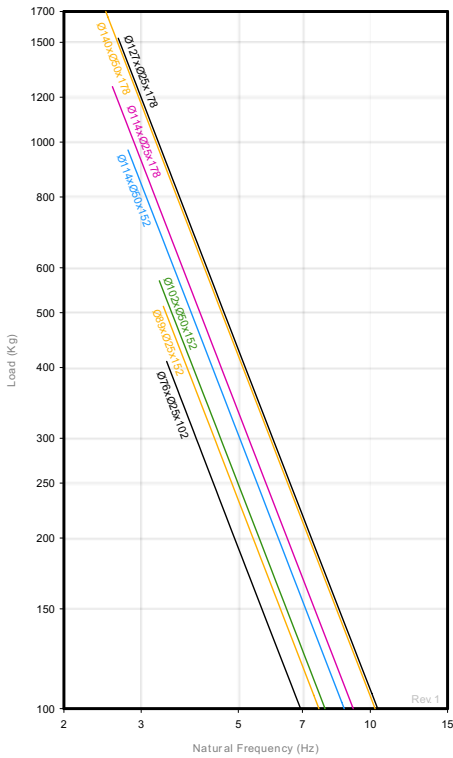
NATURAL FREQUENCY AMC MECANOCAUCHO® REINFORCED ELASTOMERIC SPRINGS Ø76 - Ø140
