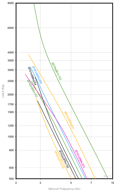
NATURAL FREQUENCY AMC MECANOCAUCHO® REINFORCED ELASTOMERIC SPRINGS Ø152 - Ø279
