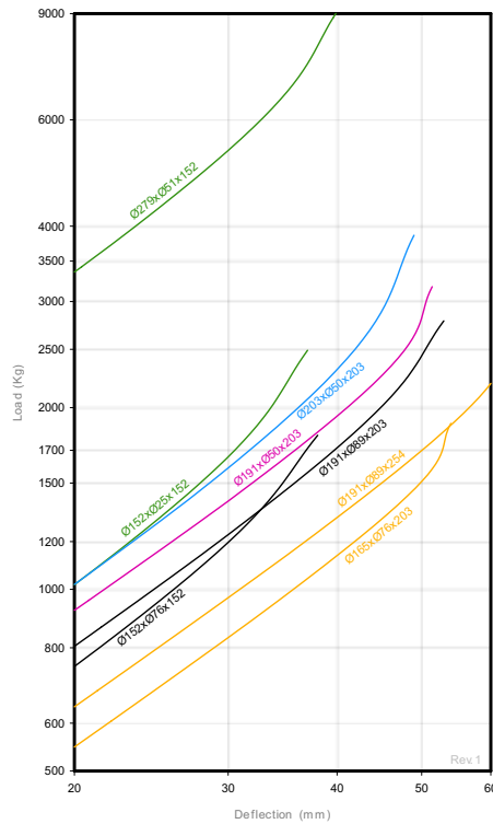
LOAD DEFLECTION GRAPH AMC MECANOCAUCHO® REINFORCED ELASTOMERIC SPRINGS Ø152 - Ø279
