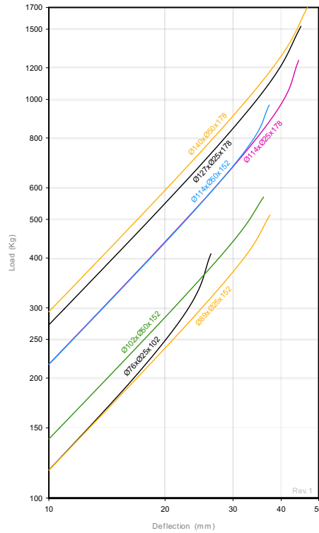
LOAD DEFLECTION GRAPH AMC MECANOCAUCHO® REINFORCED ELASTOMERIC SPRINGS Ø76 - Ø140
