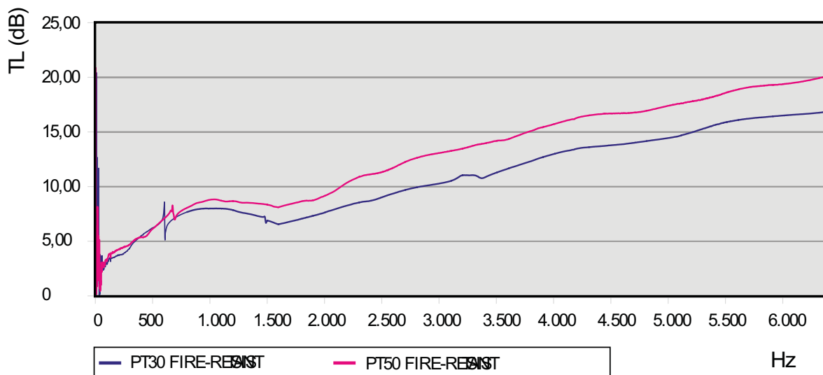
Transmission Loss (dB) PT FIRE-RESIST
