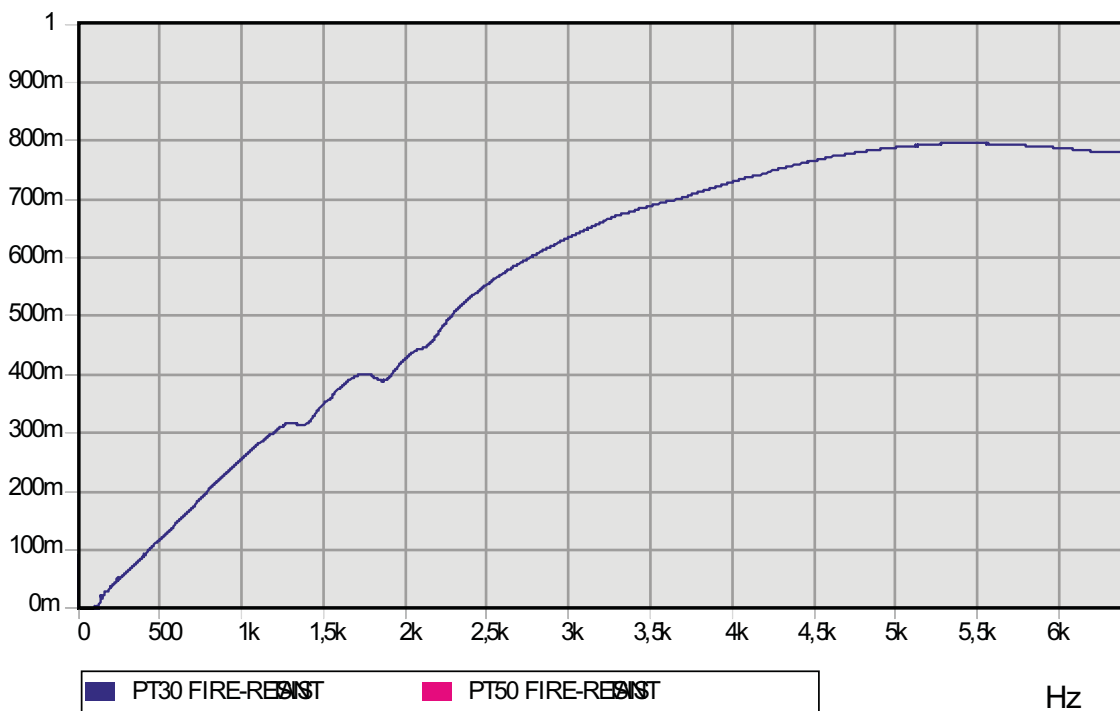
Absorption coefficient PT FIRE-RESIST
