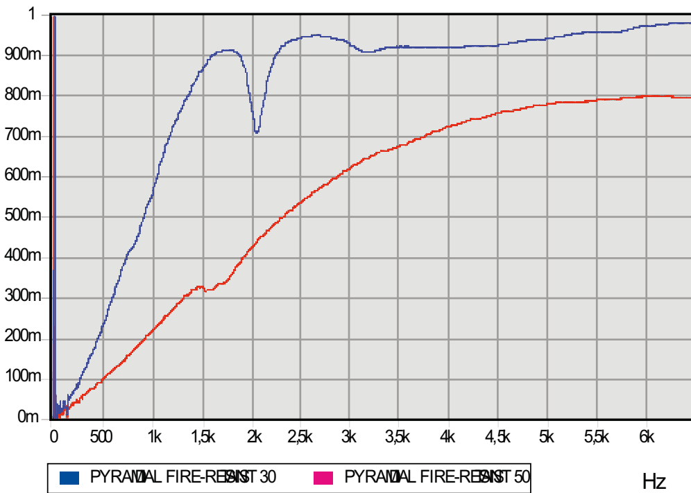
Absorption coefficient
