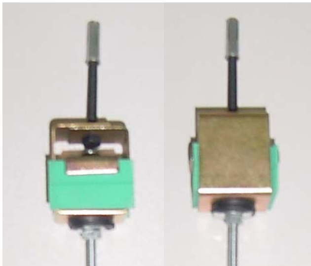
Photo 1: 'Akustik 3+Sylomer 30 Type B' ceiling support
